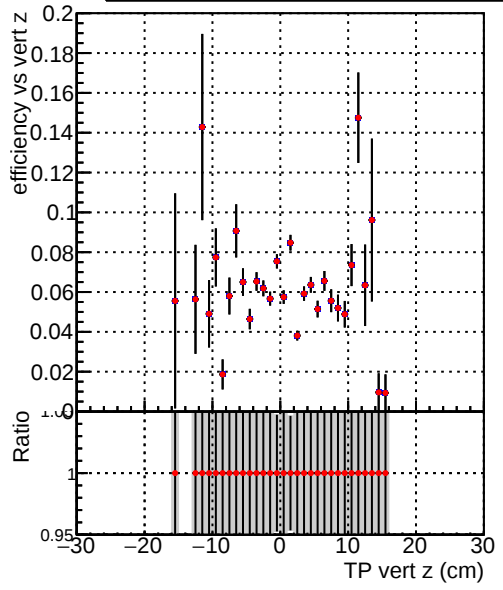
Efficiency vs vert z Legend: - ./././CMSSW_13_2_X_2023-05-08-2300/src/DQM\_TT\_mkFit-DQM\_new132 (blue line with error bars) - DQM\_TT\_mkFit-DQM\_newfast132 (red line with error bars)
