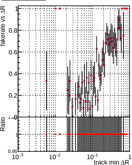
█ ● ../CMSSW_13_2_X_2023-05-08-2300/src/DQM_TT_mkFit-DQM_new132 — ● DQM_TT_mkFit-DQM_newfast132
