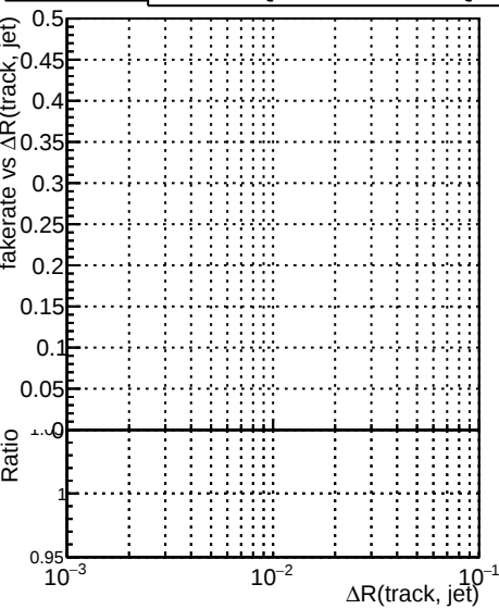
█ ● ../CMSSW_13_2_X_2023-05-08-2300/src/DQM_TT_mkFit-DQM_new132 — ● DQM_TT_mkFit-DQM_newfast132
