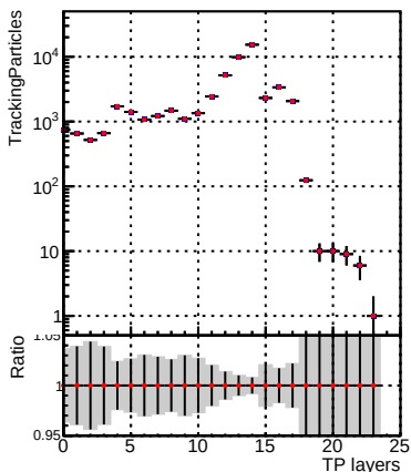
N of sim —●— DQM_TT_mkFit-DQM_newfast132
