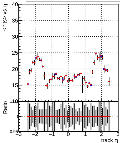
./../CMSSW_13_2_X_2023-05-08-2300/src/DQM_TT_mkFit-DQM_new132 mean hits DQM_TT_mkFit-DQM_newfast132
