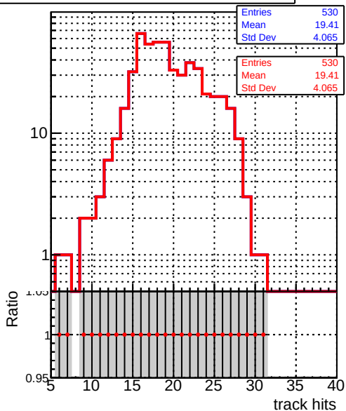
./../CMSSW_13_2_X_2023-05-08-2300/src/DQM_TT_mkFit-DQM_new132 mean hits DQM_TT_mkFit-DQM_newfast132
