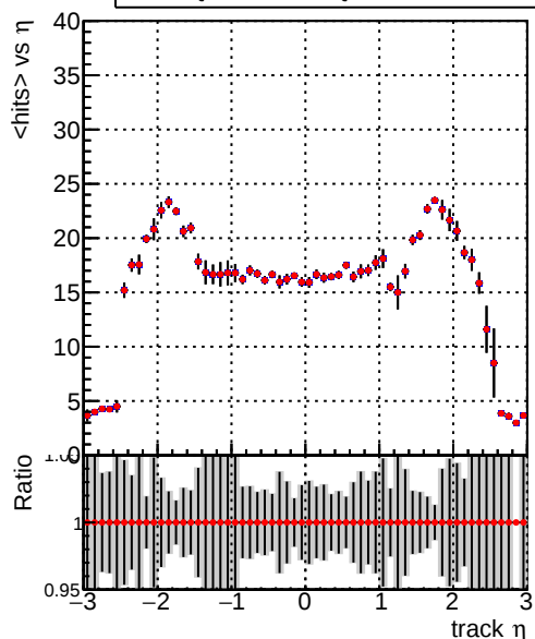
./../CMSSW_13_2_X_2023-05-08-2300/src/DQM_TT_mkFit-DQM_new132 mean hit DQM_TT_mkFit-DQM_newfast132
