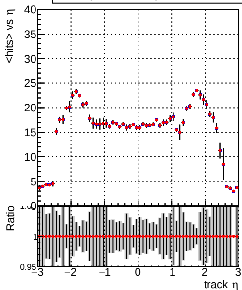
././CMSSW_13_2_X_2023-05-08-2300/src/DQM_TT_mkFit-DQM_new132 mean hit
