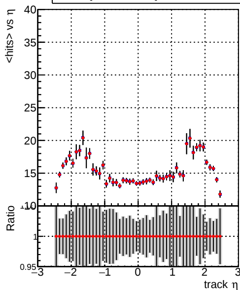
mean hits vs \eta ././CMSSW_13_2_X_2023-05-08-2300/src/DQM_TT_mkFit-DQM_new132 DQM_TT_mkFit-DQM_newfast132
