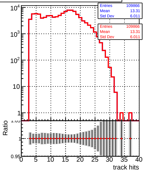
././CMSSW_13_2_X_2023-05-08-2300/src/DQM_TT_mkFit-DQM_new132 mean hit DQM_TT_mkFit-DQM_newfast132
