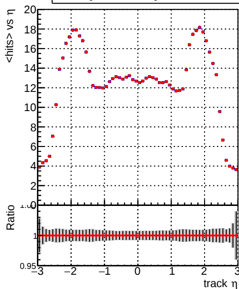
././CMSSW_13_2_X_2023-05-08-2300/src/DQM_TT_mkFit-DQM_new132 mean hit DQM_TT_mkFit-DQM_newfast132
