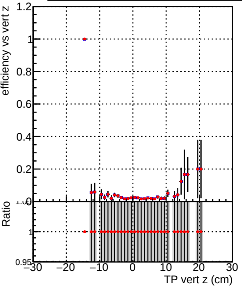
Efficiency vs TP vert z (cm) Legend: - ././CMSSW_13_2_X_2023-05-08-2300/src/DQM_TT_mkFit-DQM_new132 (grey line with blue dots) - DQM_TT_mkFit-DQM_newfast132 (red line with red dots)
