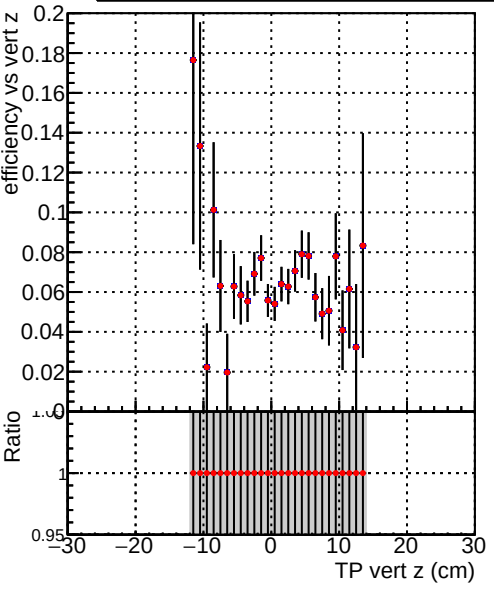
Efficiency vs vertpos Legend: Blue line with square markers: ./../CMSSW_13_2_X_2023-05-08-2300/src/DQM_TT_mkFit-DQM_new132 Red line with star markers: DQM_TT_mkFit-DQM_newfast132
