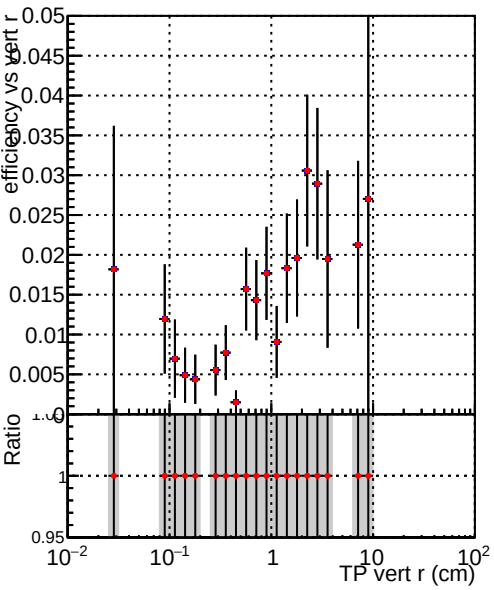
Efficiency vs vertpos Legend: ././CMSSW_13_2_X_2023-05-08-2300/src/DQM_TT_mkFit-DQM_new132 DQM_TT_mkFit-DQM_newfast132
