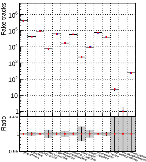
Number —●— DQM_TT_mkFit-DQM_newfast132
