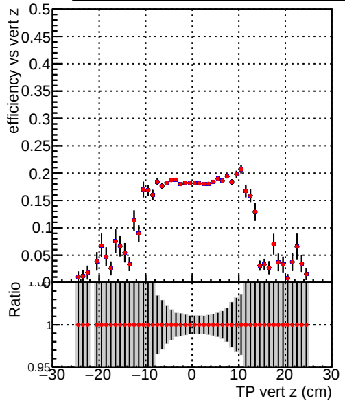
Efficiency vs TP vert z Legend: - ./././CMSSW_13\_2\_X\_2023-05-08-2300/src/DQM\_TT\_mkFit-DQM\_new132 (blue line with dots) - DQM\_TT\_mkFit-DQM\_newfast132 (red line with dots)
