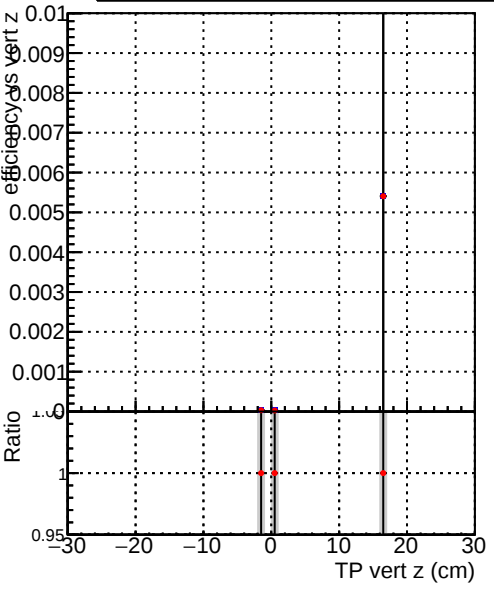
Efficiency vs. TP vert z Legend: - ■ ././CMSSW_13_2_X_2023-05-08-2300/src/DQM_TT_mkFit-DQM_new132 - ● DQM_TT_mkFit-DQM_newfast132
