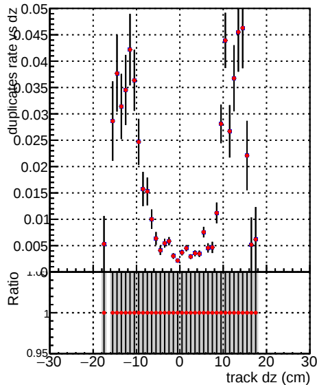
./../CMSSW_13_2_X_2023-05-08-2300/src/DQM_TT_mkFit-DQM_new132
