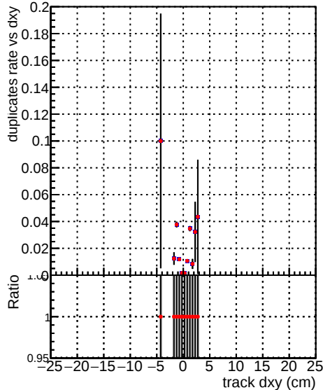
./../CMSSW_13_2_X_2023-05-08-2300/src/DQM_TT_mkFit-DQM_new132
