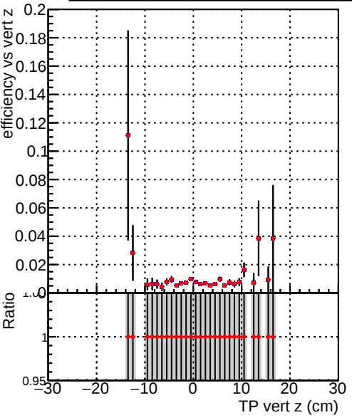
Efficiency vs. TP vert z (cm) for ./J./CMSSW_13_2_X_2023-05-08-2300/src/DQM_TT_mkFit-DQM_new132 (blue line) and DQM_TT_mkFit-DQM_newfast132 (red line).
