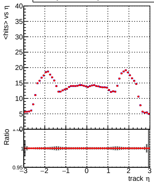
mean hits vs \eta ././CMSSW_13_2_X_2023-05-08-2300/src/DQM_TT_mkFit-DQM_new132 DQM_TT_mkFit-DQM_newfast132
