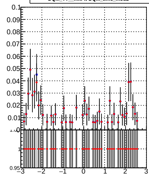
DQM\_TT\_mkFit-DQM\_time\_orig2 DQM\_TT\_mkFit-DQM\_time\_mod2
