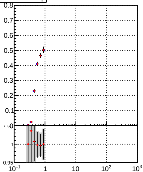
DQM\_TT\_mkFit-DQM\_time\_orig2 DQM\_TT\_mkFit-DQM\_time\_mod2
