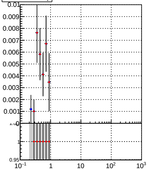
—•— DQM_TT_mkFit-DQM_time_orig2 —•— DQM_TT_mkFit-DQM_time_mod2
