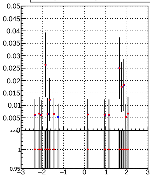
—•— DQM_TT_mkFit-DQM_time_orig2 —•— DQM_TT_mkFit-DQM_time_mod2
