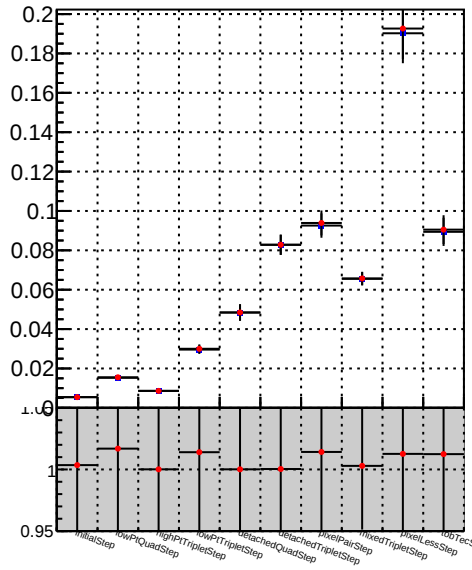
Average real time / selected HP track by algoMask
