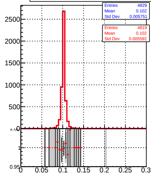
Recons Legend: DQM_TT_mkFit-DQM_time_orig2 (blue line with markers), DQM_TT_mkFit-DQM_time_mod2 (red line with markers)
