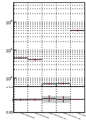
N of reco track vs. \chi^2 for different fit models
