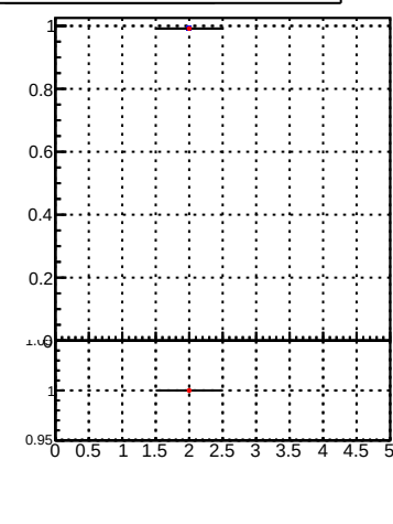
fake+duplicates vs 3D layers
