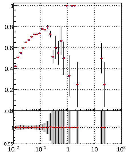
—•— DQM_TT_mkFit-DQM_time_orig2 —•— DQM_TT_mkFit-DQM_time_mod2
