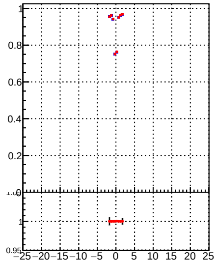
—•— DQM TT mkFit-DQM_time_orig2 —•— DQM TT mkFit-DQM_time_mod2
