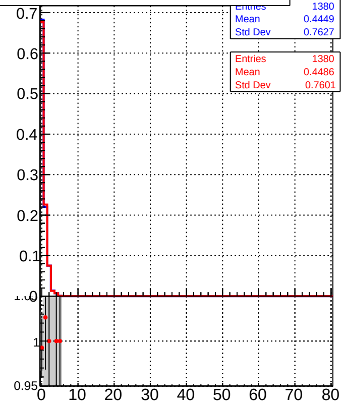
Legend: ■ DQM_TT_mkFit-DQM_time_orig2 ● DQM_TT_mkFit-DQM_time_mod2
