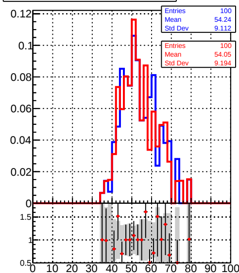
ReconstructedAllAssoc2Gen_NumVertices
