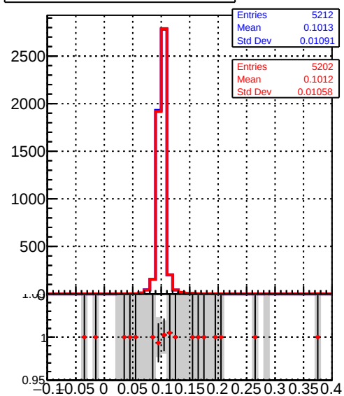
ReconstructedAllAssoc2Gen_X
