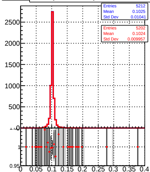
ReconstructedAllAssoc2Gen_X
