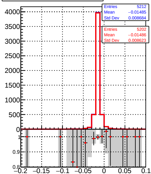
ReconstructedAllAssoc2Gen_Y
