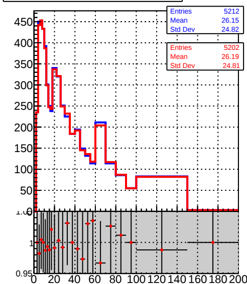
ReconstructedAllAssoc2Gen_NumTracks
