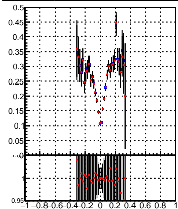
—●— DQM_TT_mkFit-DQM_time_orig2 —●— DQM_TT_mkFit-DQM_time_mod2
