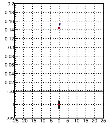
—●— DQM_TT_mkFit-DQM_time_orig2 —●— DQM_TT_mkFit-DQM_time_mod2
