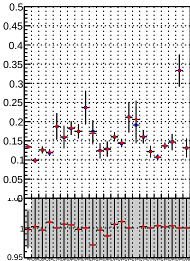
Fake rate vs. — DQM TT mkFit-DQM_time_orig2 — DQM TT mkFit-DQM_time_mod2
