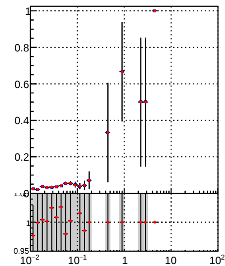
—•— DQM_TT_mkFit-DQM_time_orig2 —•— DQM_TT_mkFit-DQM_time_mod2
