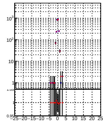
DQM_TT_mkFit-DQM_time_orig2 DQM_TT_mkFit-DQM_time_mod2
