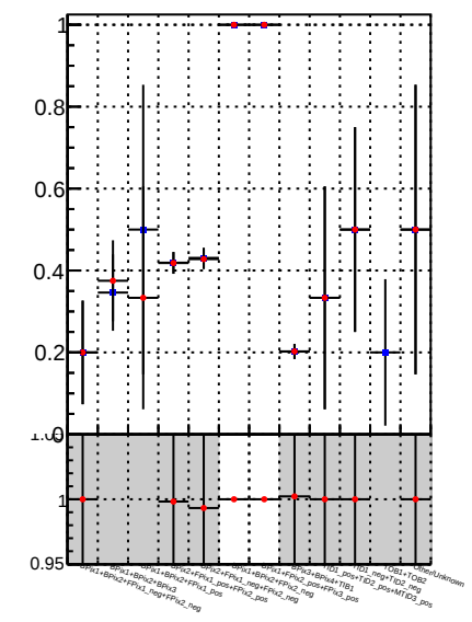
Fake rate vs. —●— DQM_TT_mkFit-DQM_time_orig2 —●— DQM_TT_mkFit-DQM_time_mod2
