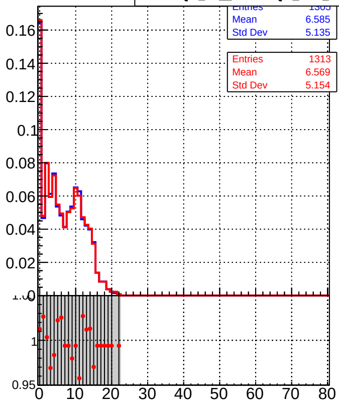
— DQM_TT_mkFit-DQM_time_orig2 — DQM_TT_mkFit-DQM_time_mod2
