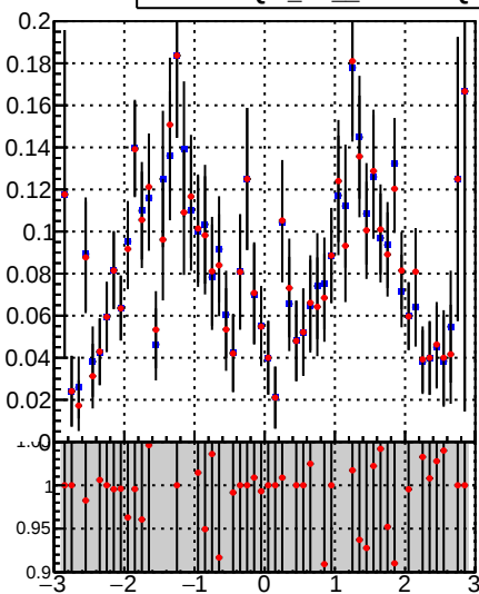
—■— DQM_TT_mkFit-DQM_time_orig2 —●— DQM_TT_mkFit-DQM_time_mod2
