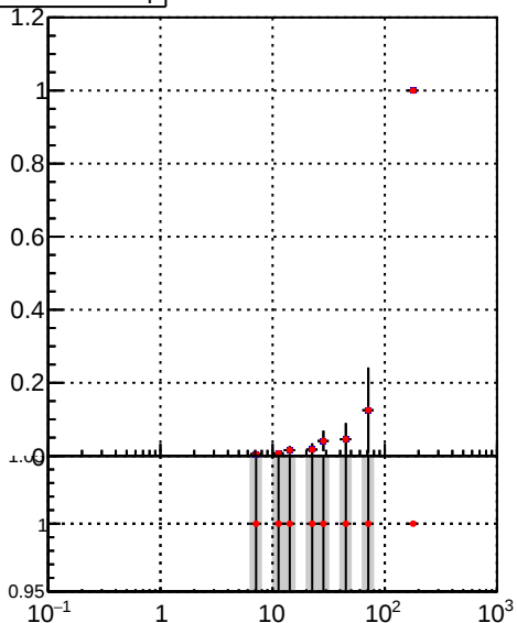
—•— DQM_TT_mkFit-DQM_time_orig2 —•— DQM_TT_mkFit-DQM_time_mod2
