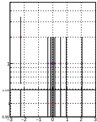
N of reco track vs \eta DQM_TT_mkFit-DQM_time_orig2 DQM_TT_mkFit-DQM_time_mod2
