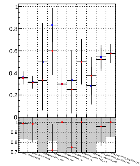
Fake rate vs. DQM_TT_mkFit-DQM_time_orig2 DQM_TT_mkFit-DQM_time_mod2
