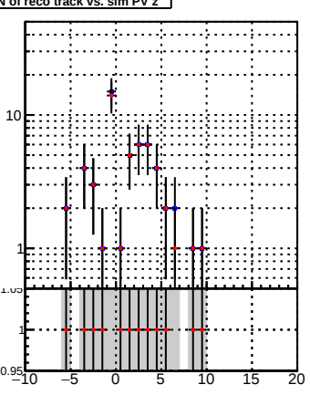
N of reco track vs. sim PV z
