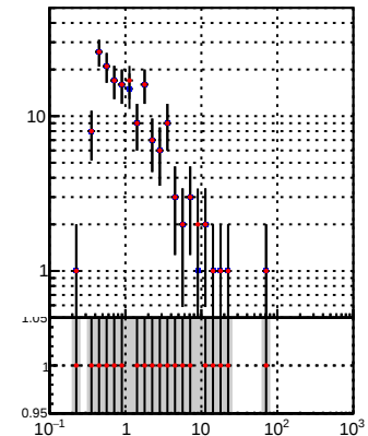
N of reco track vs \eta pT eta —•— DQM TT mkFit-DQM_time_orig2 —•— DQM TT mkFit-DQM_time_mod2
