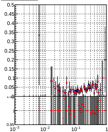
Fake rate vs dr Legend: —•— DQM_TT_mkFit-DQM_time_orig2 —•— DQM_TT_mkFit-DQM_time_mod2
