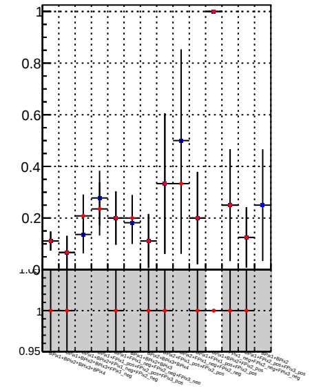
Fake rate vs. — DQM_TT_mkFit-DQM_time_orig2 — DQM_TT_mkFit-DQM_time_mod2
