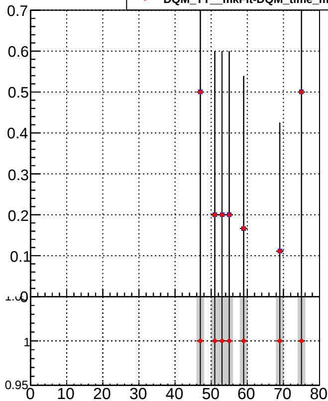
■ DQM_TT_mkFit-DQM_time_orig2 ● DQM_TT_mkFit-DQM_time_mod2
