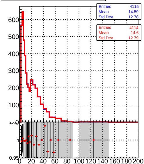
ReconstructedAllAssoc2Gen_NumTracks
