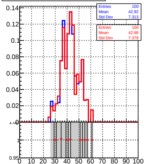
ReconstructedAllAssoc2Gen_NumVertices
