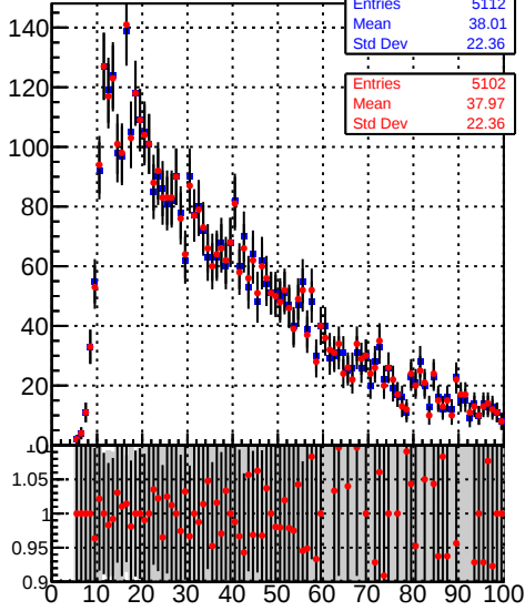
Uncertainty x Coordinate (tagged Vtx) vs Uncertainty x Coordinate (other Vtx)
