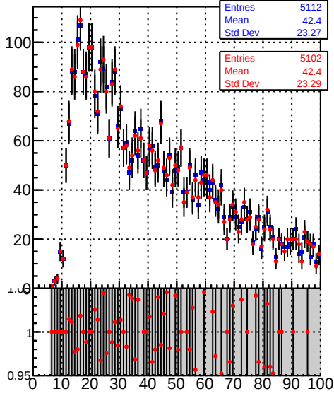
Uncertainty z Coordinate (other Vtx)
