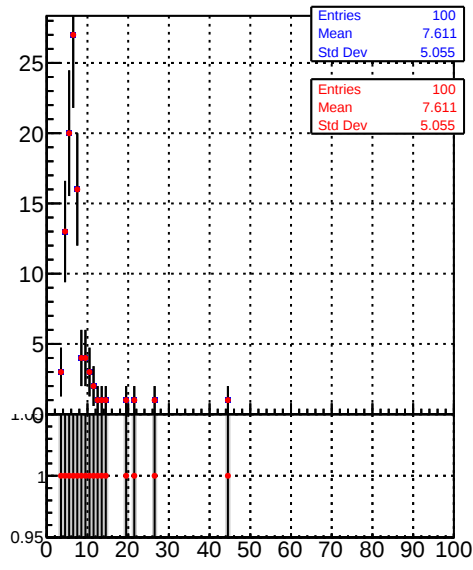
Uncertainty x Coordinate (tagged Vtx)
