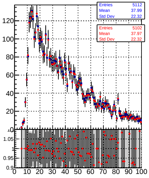
Uncertainty x Coordinate (other Vtx)
