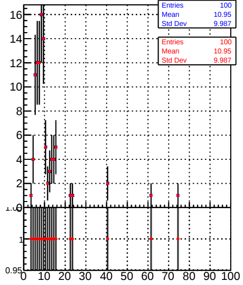
Uncertainty z Coordinate (tagged Vtx)
