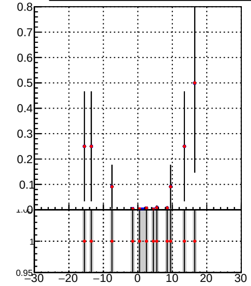
Efficiency vs. sim PV z Legend: — DQM_TT_mkFit-DQM_time_orig2 — DQM_TT_mkFit-DQM_time_mod2
