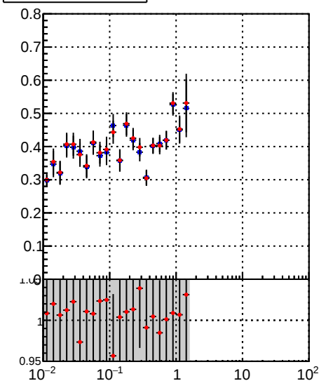
—•— DQM_TT_mkFit-DQM_time_orig2 —•— DQM_TT_mkFit-DQM_time_mod2
