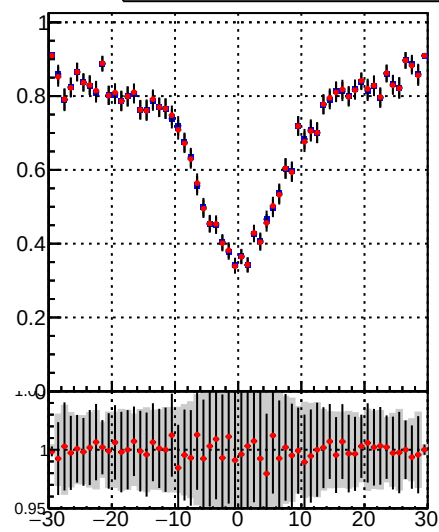
—•— DQM_TT_mkFit-DQM_time_orig2 —•— DQM_TT_mkFit-DQM_time_mod2
