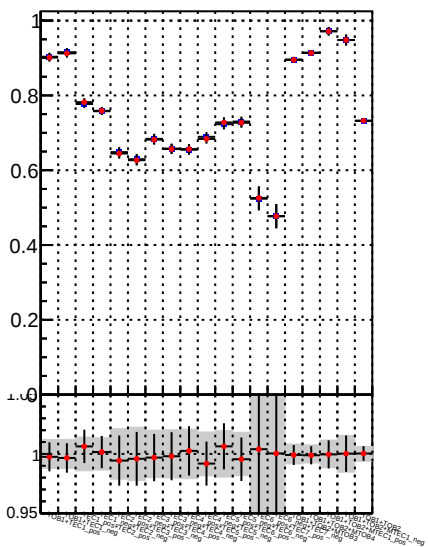
Fake rate vs. DQM_TT_mkFit-DQM_time_orig2 DQM_TT_mkFit-DQM_time_mod2
