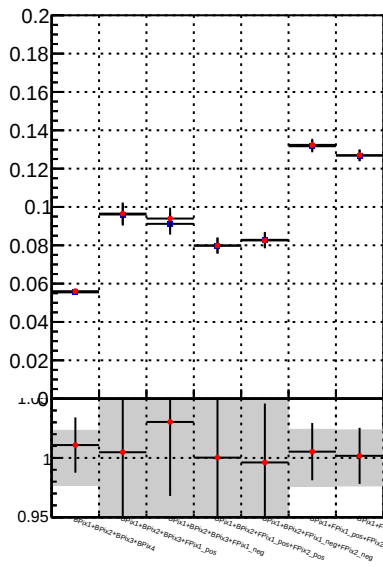
Fake rate vs. — DQM TT mkFit-DQM_time_orig2 — DQM TT mkFit-DQM_time_mod2
